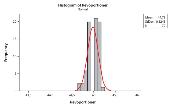
4b. Weight distribution of low pressure portioned products.
